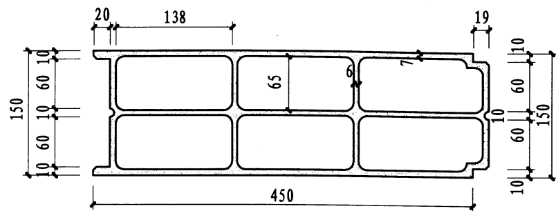
PB-ZK1545-6
