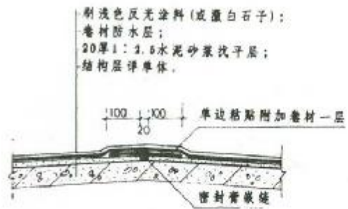
2 卷材屋面屋脊分格缝
