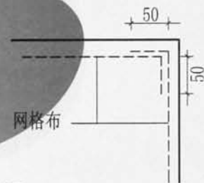
B 阴角网格布搭接
